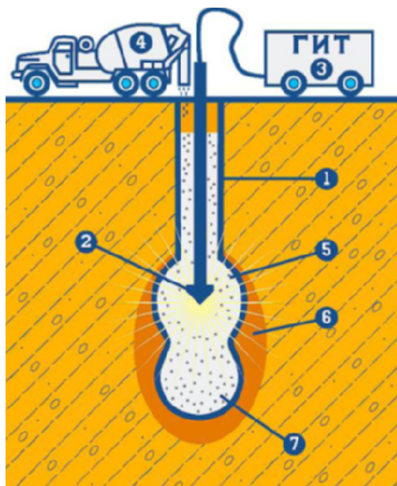
Fig. 1. Recharge impulse technology in RIT-pile:
